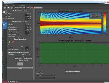
intermediate ADO
